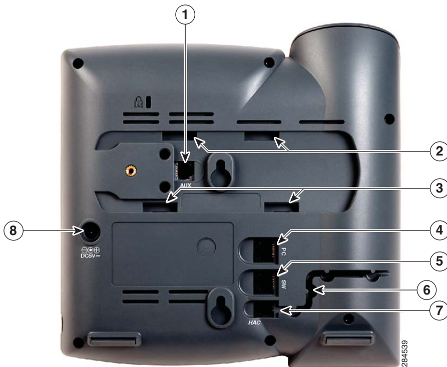
Figure 1 Phone Connections
